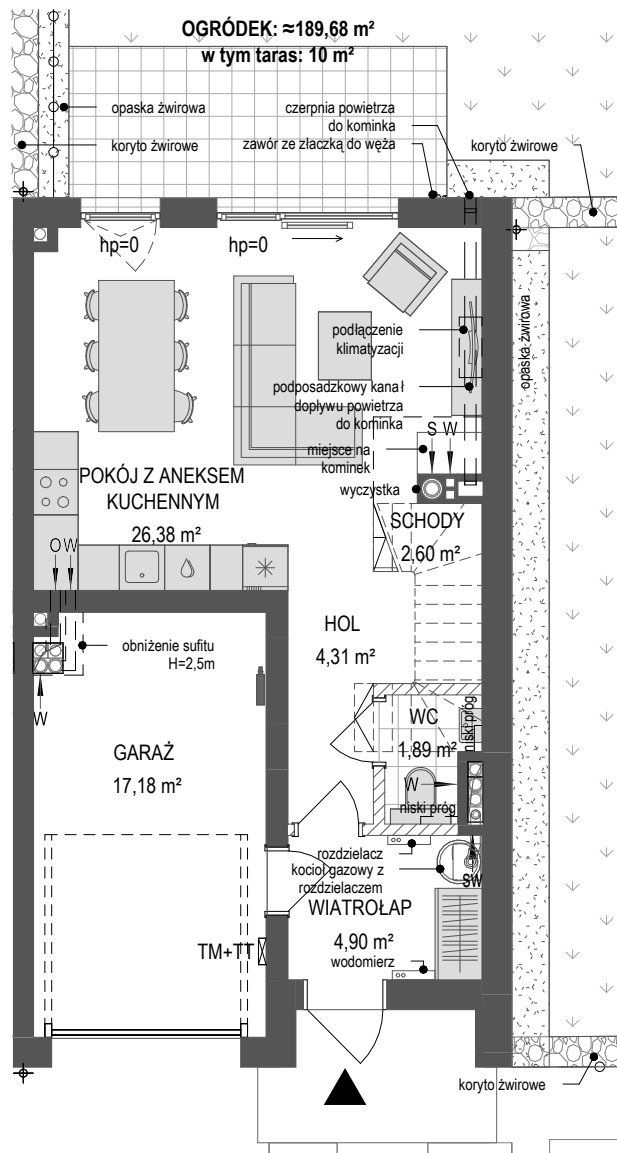
PARTER 57,26 m 2
